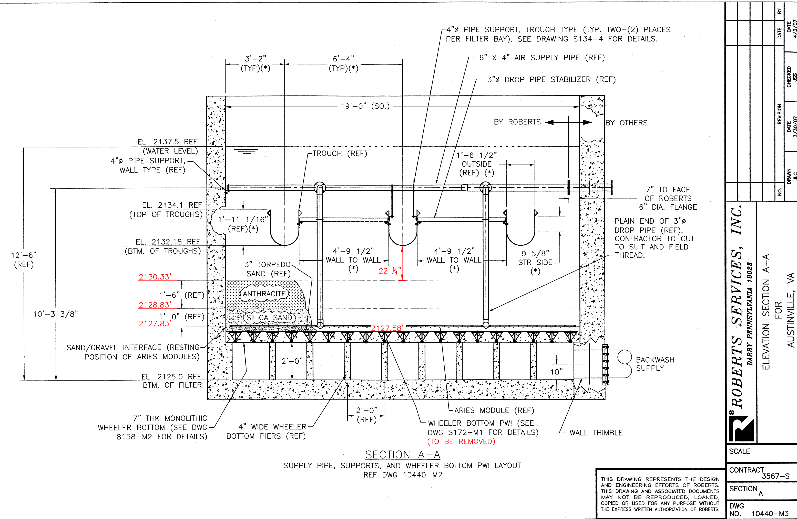
EXISTING FILTER SECTION WITH PWI INSERT UNDERDRAIN N.T.S.
