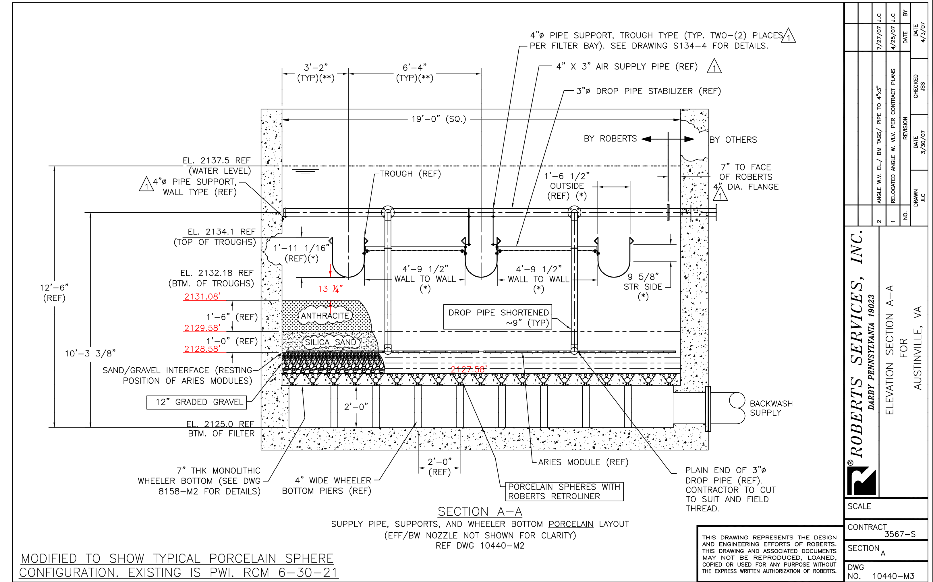
PROPOSED FILTER SECTION WITH PORCELAIN SPHERE UNDERDRAIN N.T.S.
